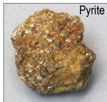
Pyrite
